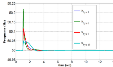
Fig. 4. Frequency graph f(t) before WPP Jeneponto injection
