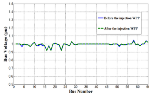
Fig. 2. Profile of voltage before and after WPP Jeneponto injection
