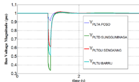
Fig. 5. Voltage graph f(t) before WPP Jeneponto injection.
