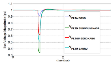
Fig. 8. Voltage graph f(t) after WPP Jeneponto injection
