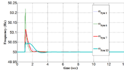
Fig. 7. Frequency graph f(t) after WPP Jeneponto injection
