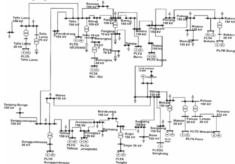
Fig. 1. Single line diagram SULSELBAR system.
